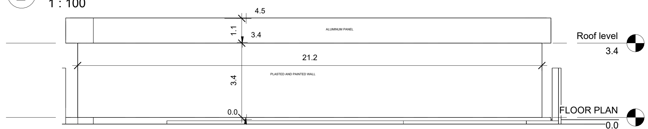
3 REAR ELEVATION 1 : 100
