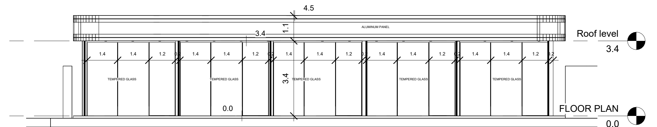
2 FRONT ELEVATION 1 : 100
