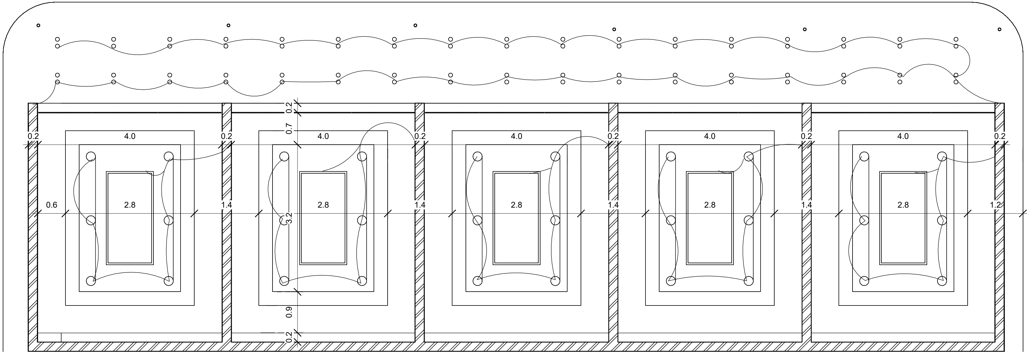
1 1:50 INSTALLATION OF LIGHT AND SWITCH
